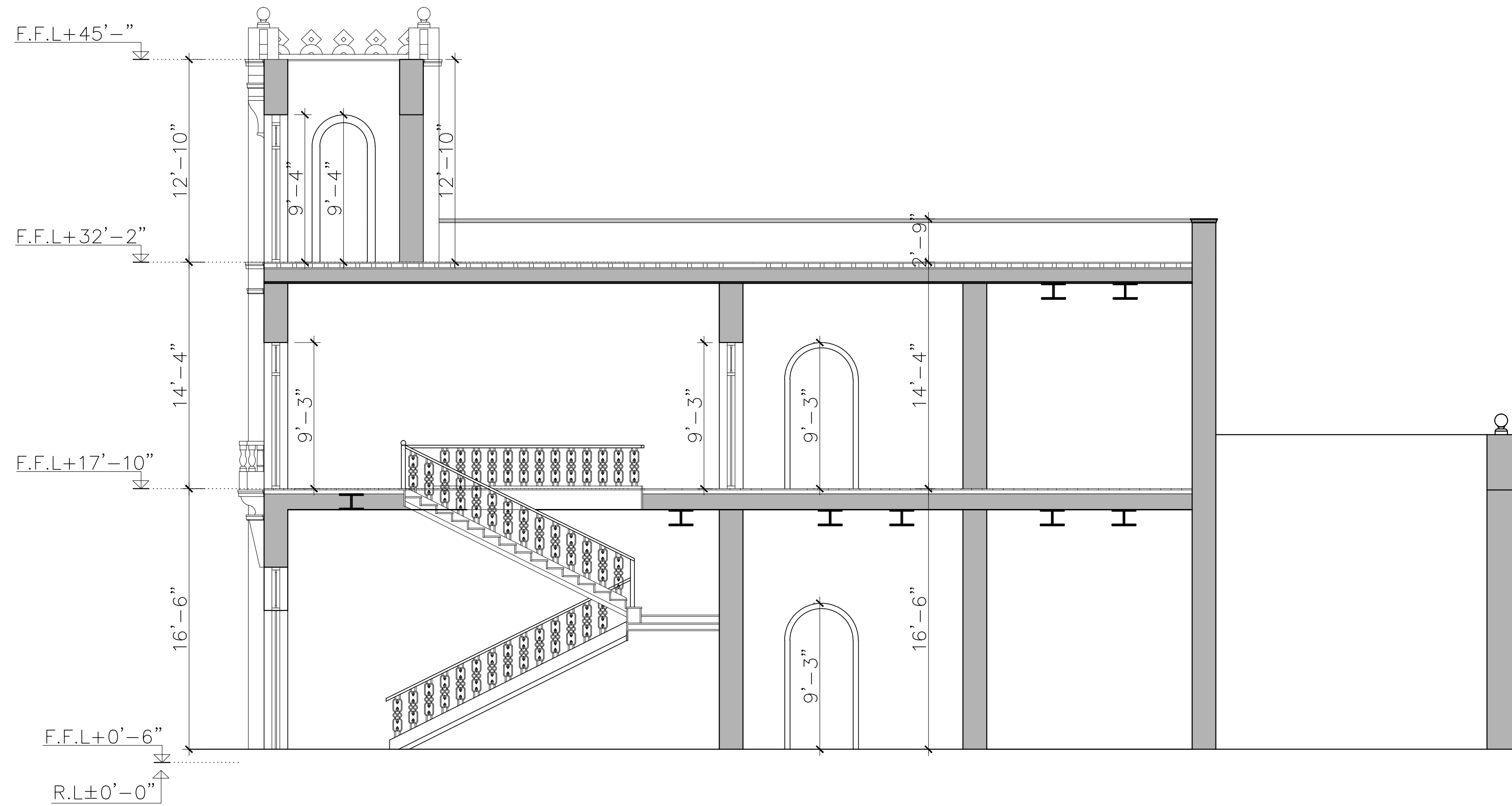
SECTION- A-A
