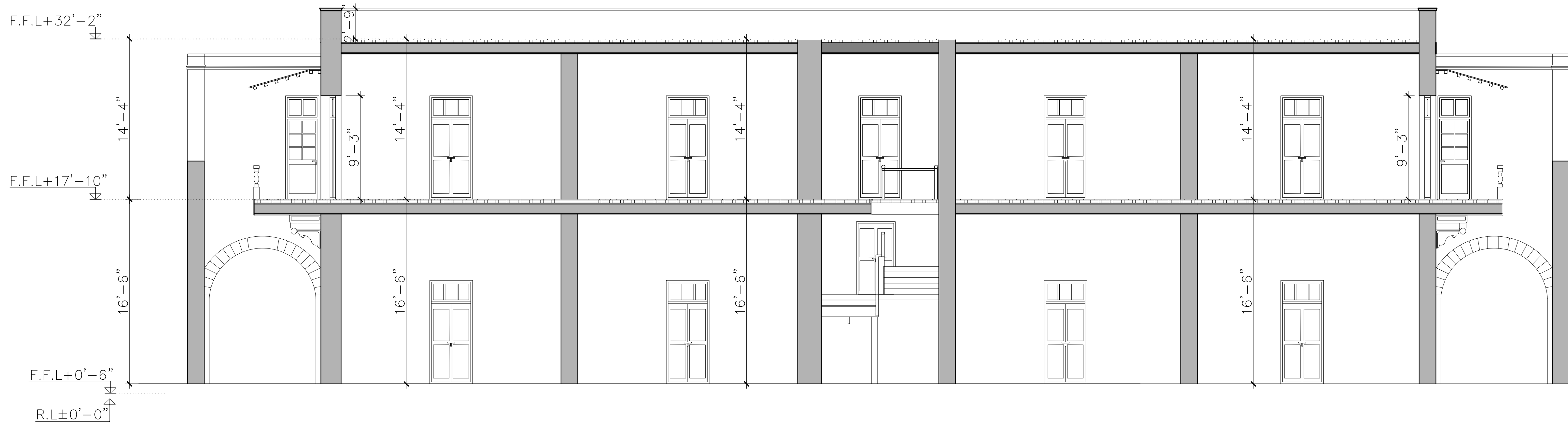
SECTION- B-B
