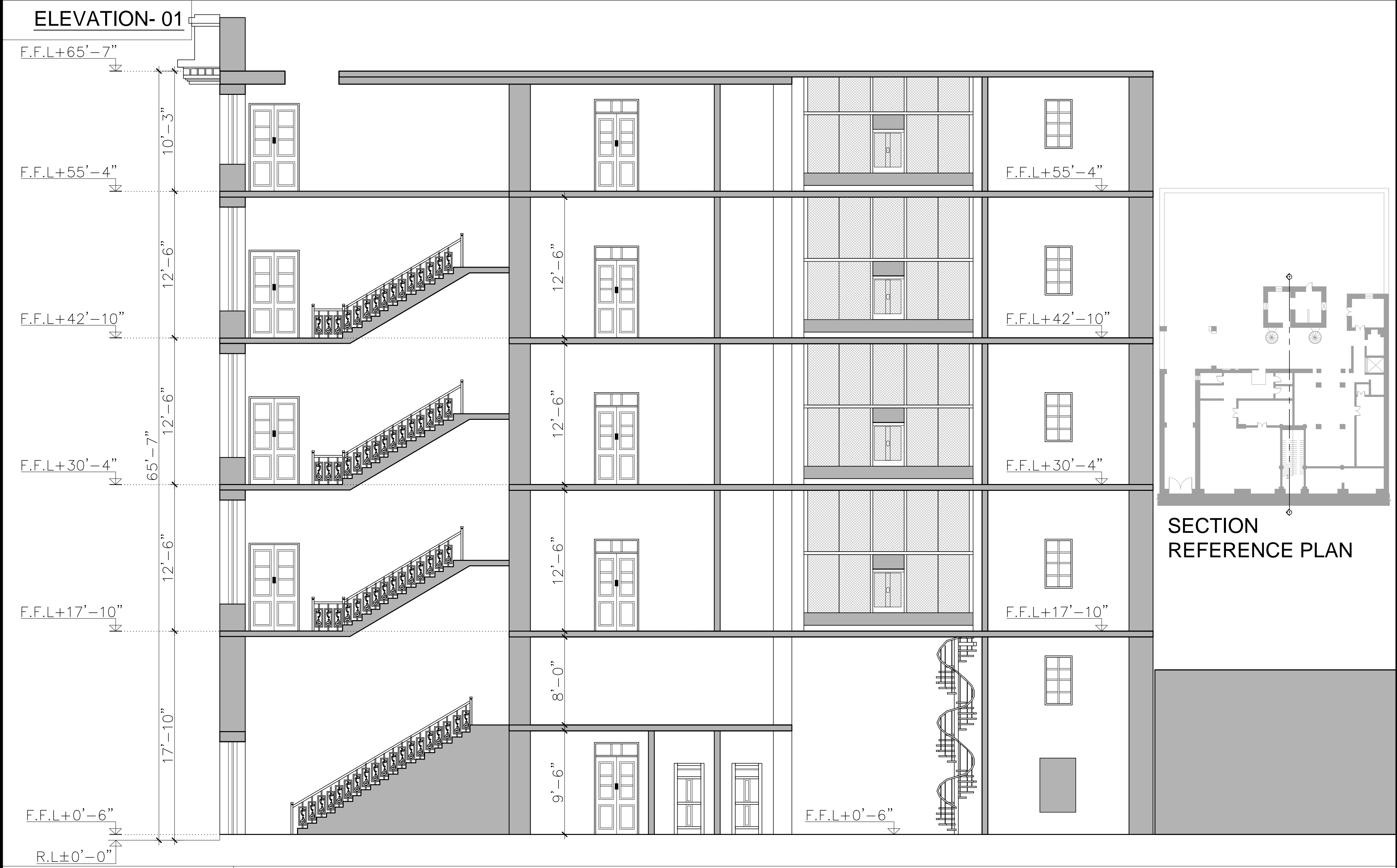
SECTION- Y-Y
