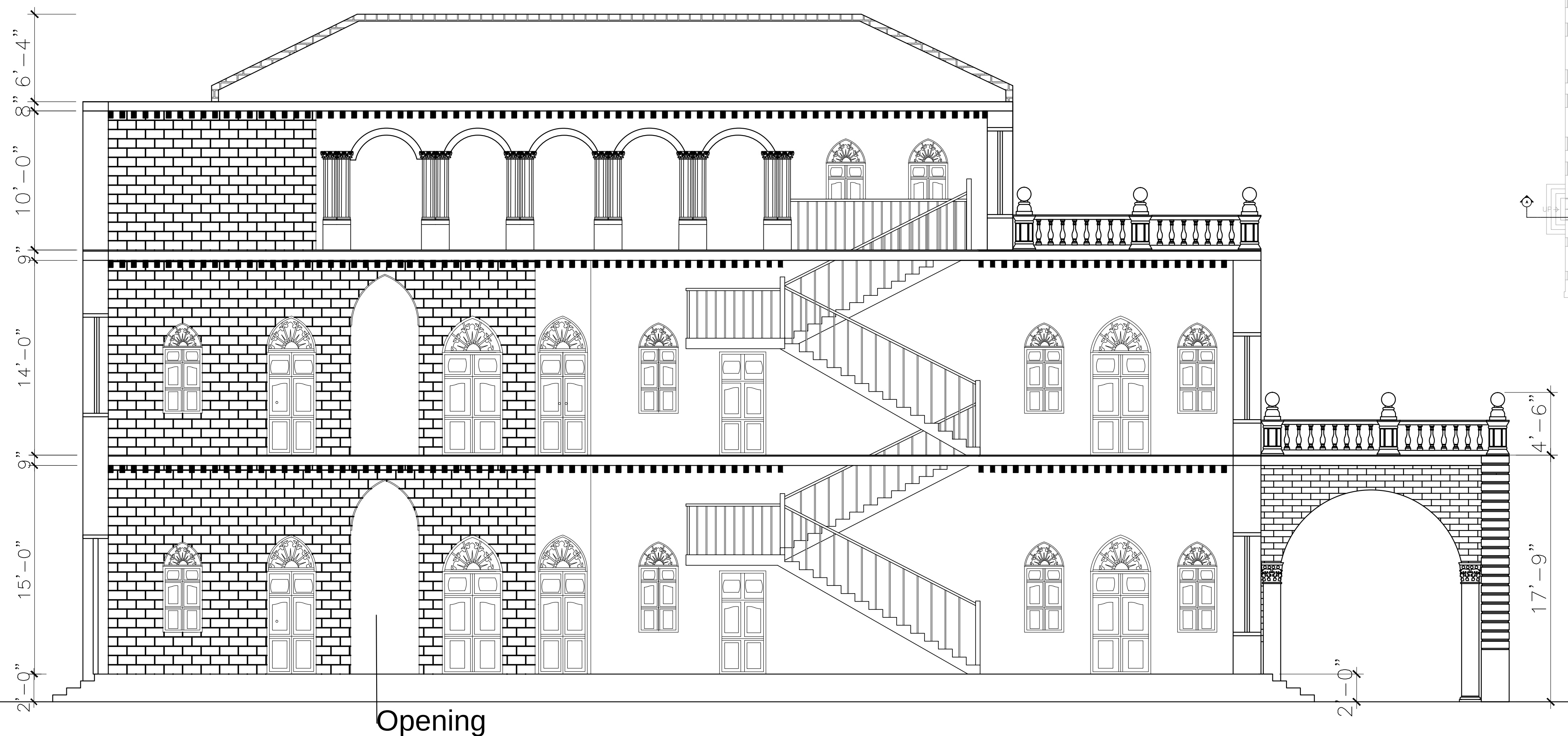
SECTION- A-A
