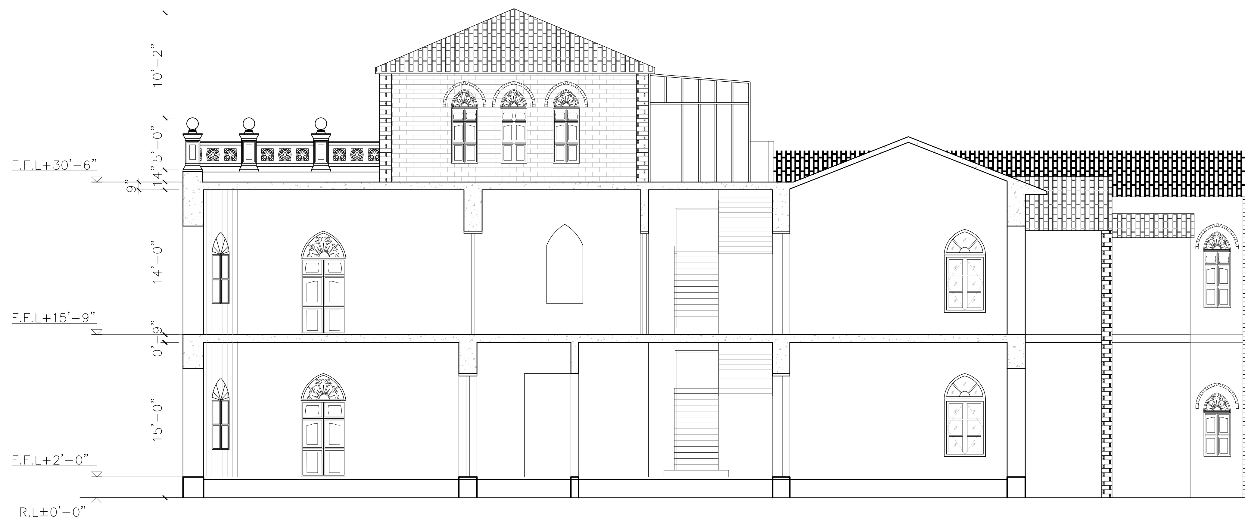
SECTION- B-B
